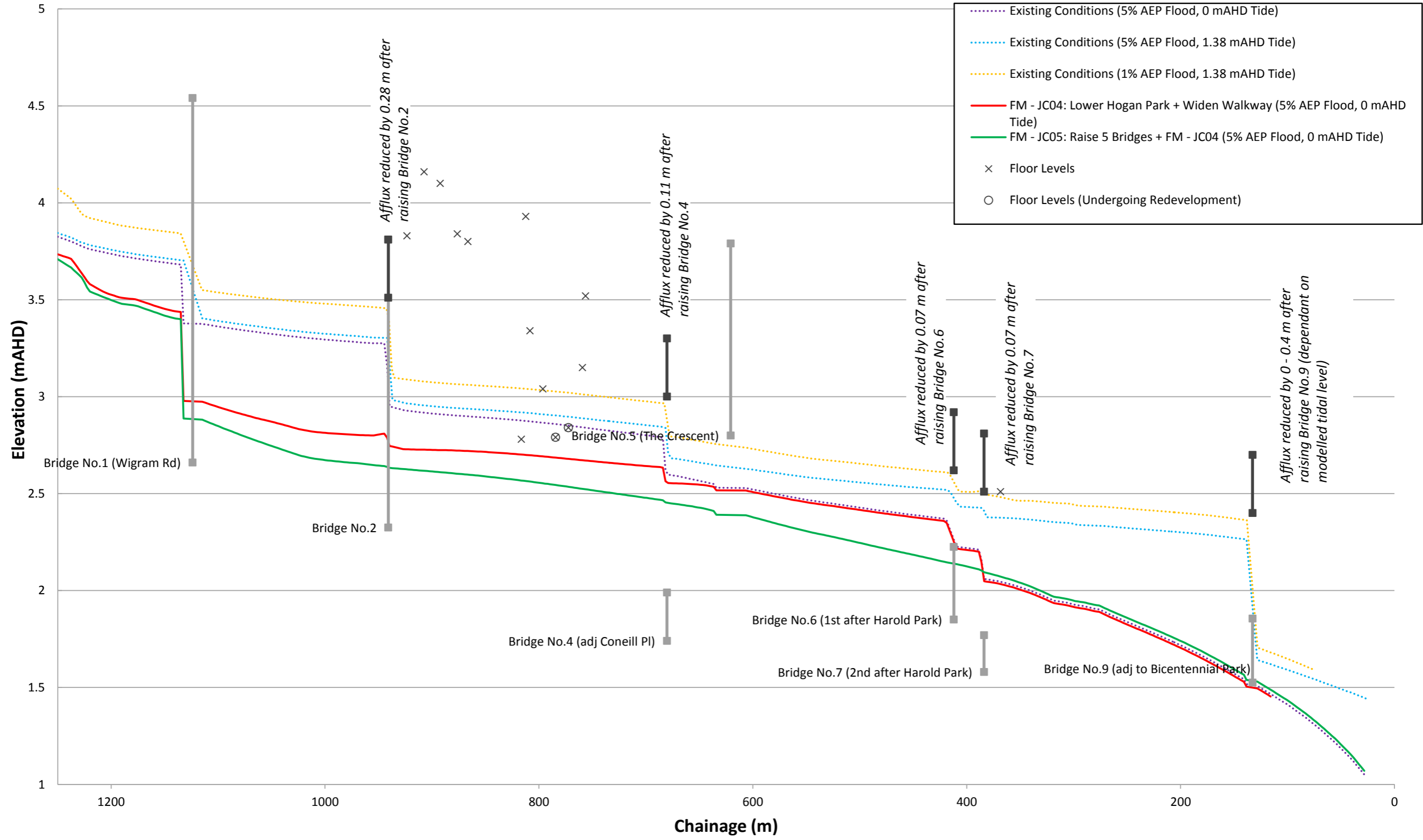
FIGURE 36 OPTION FM - JC04 & FM - JC05 LOWERING OF HOGAN PARK & BRIDGE RAISING PEAK FLOOD LEVEL PROFILES 5% and 1% AEP DESIGN FLOOD EVENTS
